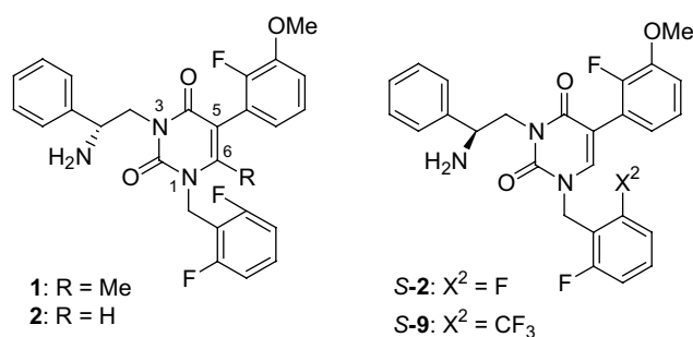
Figure 1. Structure of uracil analogues.
