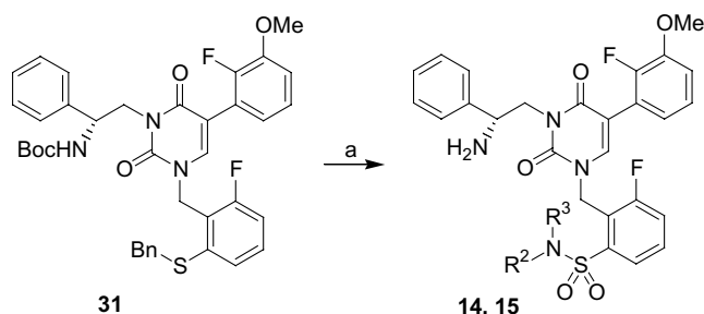
Scheme 3. Reagents and conditions: (a) i. NCS/DCM; ii. R^2R^3\text{NH} ; iii. TFA/ \text{CH}_2\text{Cl}_2 , 40–50% overall yields.
