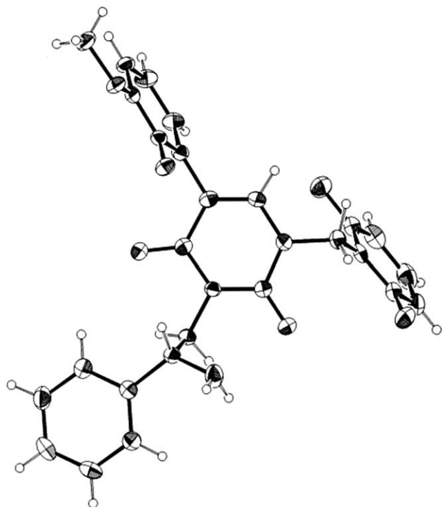
Figure 2. ORTEP drawing of the X-ray structure of compound 2 . 16
