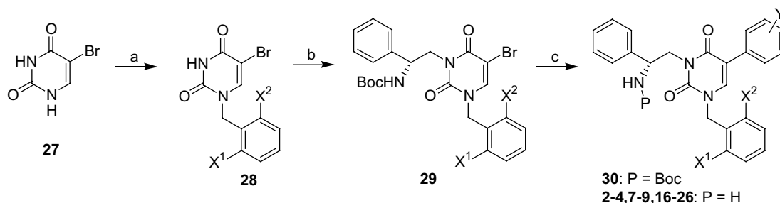
Scheme 1. Reagents and conditions: (a) BSA/ArCH 2 Br/ACN/80 °C, 85%; (b) ( R )-PhCH(NHBoc)CH 2 OH/DEAD/Ph 3 P/THF, 91%; (c) ArB(OH) 2 /Pd(0)/Na 2 CO 3 ; then TFA/CH 2 Cl 2 , 60–95%.
