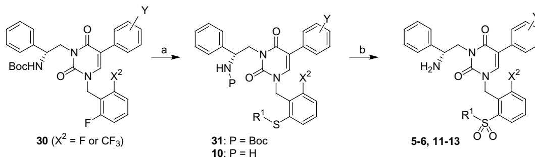
Scheme 2. Reagents and conditions: (a) R^1\text{SNa}/\text{DMF}/100\text{ }^\circ\text{C} , 98% ( R^1 = \text{Me} ); (b) oxone/acetone/ \text{H}_2\text{O} , 90%; then TFA/ \text{CH}_2\text{Cl}_2 , 90% ( R^1 = \text{Me} ).
